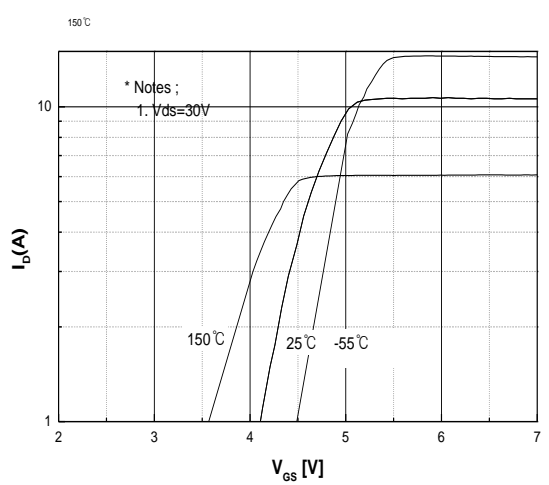
Fig.5 Transfer Characteristics
